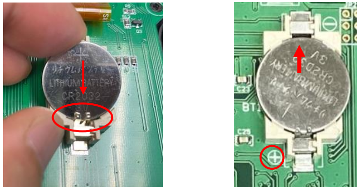
Figure 10. Install a CR2032 battery
